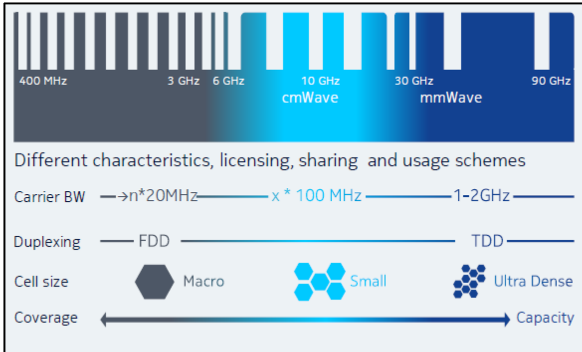
Figure 15: Characteristics of Different Bands 33
