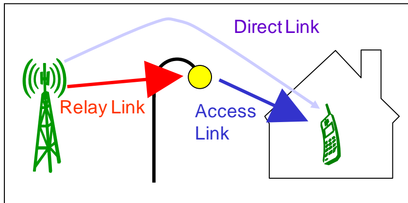
Figure 73: LTE-Advanced Relay 155
