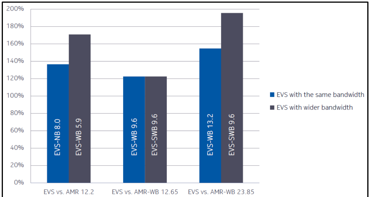
Figure 80: EVS Voice Capacity Compared to AMR and AMR-WB 173
