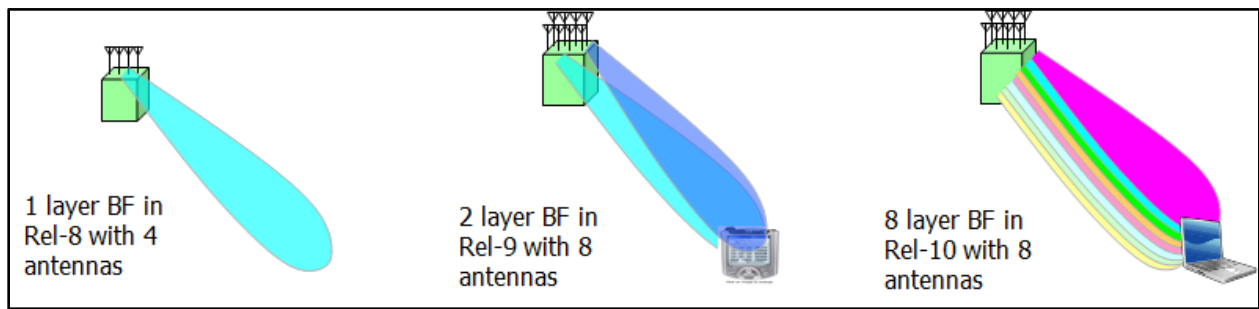
Figure 60: Single-User MIMO 135
