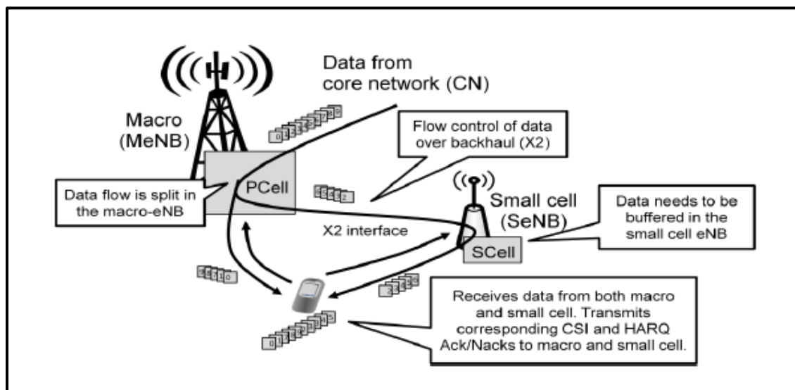
Figure 90: Dual Connectivity 183
