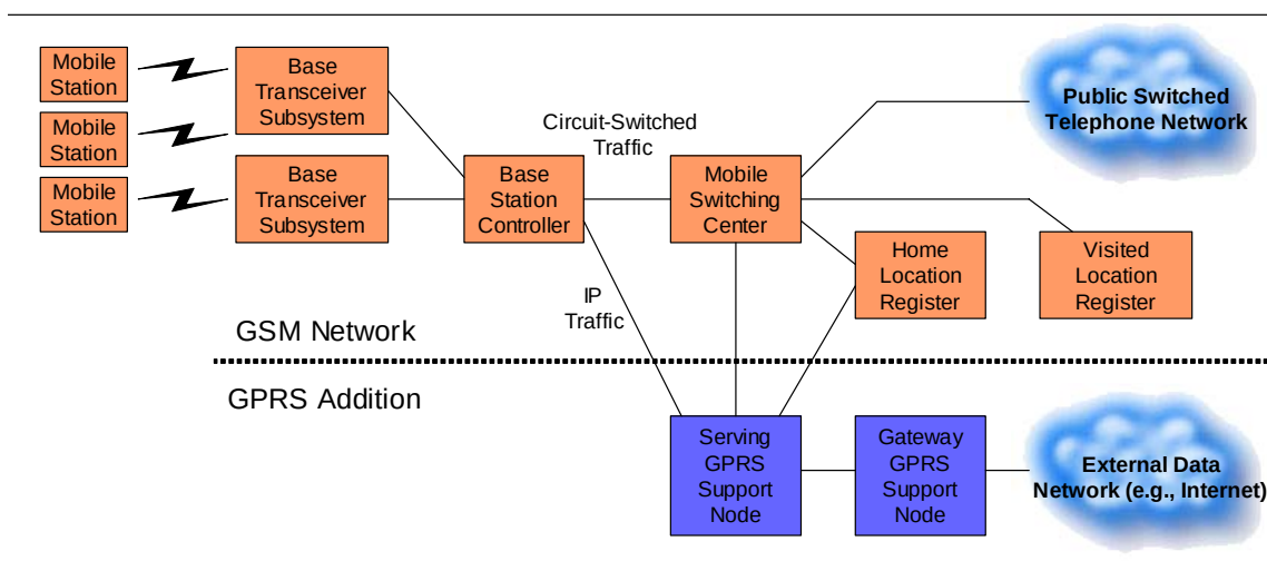
Figure 2: GSM / GPRS Architecture
